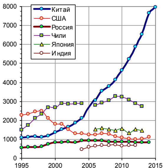
Рис. 1.118, в. Производство рафинированной меди, тыс. т. Источники: Росстат; United Nations Statistics Division, UN Industrial Commodity Statistics Database; The World Copper Factbook; USGS, Mineral Resources Program, Mineral Statistics and Commodity Information; Reserve Bank of India; National Bureau of Statistics of China.
